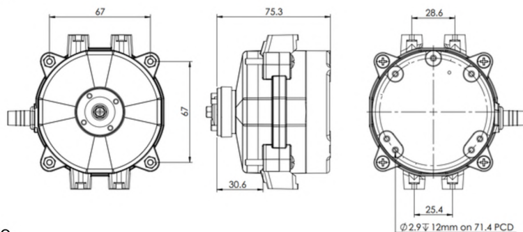
EXTERNAL VIEWS
